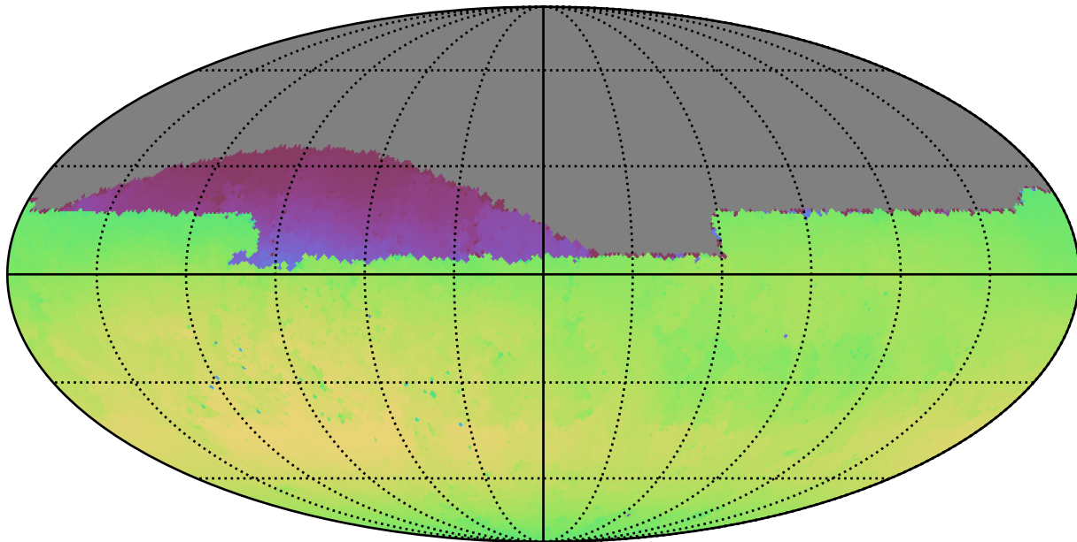
weather_cloudso4v3.4_10yrs Yr1 all bands: Max skyBrightness
