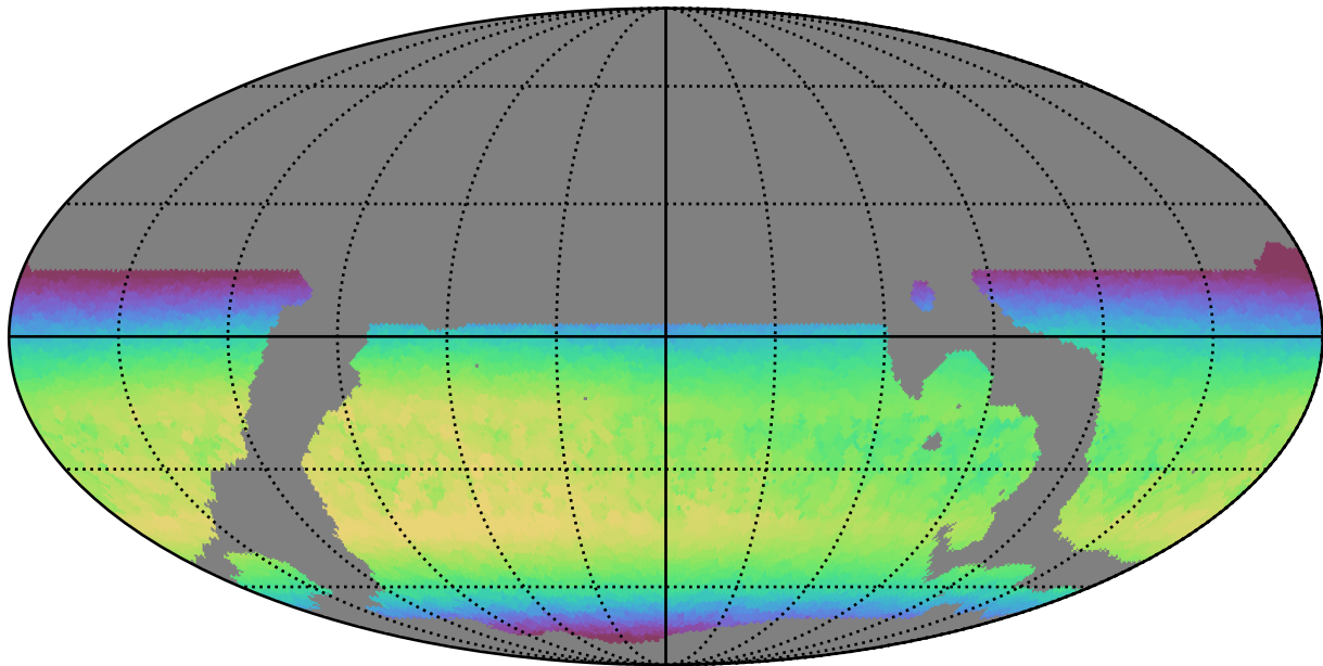
weather_cloudso4v3.4_10yrs WFD z band: Max skyBrightness
