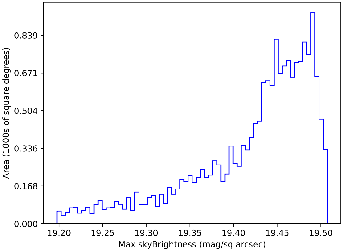
weather_cloudso4v3.4_10yrs WFD z band: Max skyBrightness
