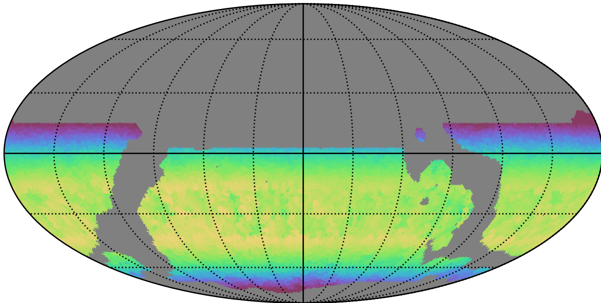
weather_cloudso4v3.4_10yrs WFD y band: Max skyBrightness
