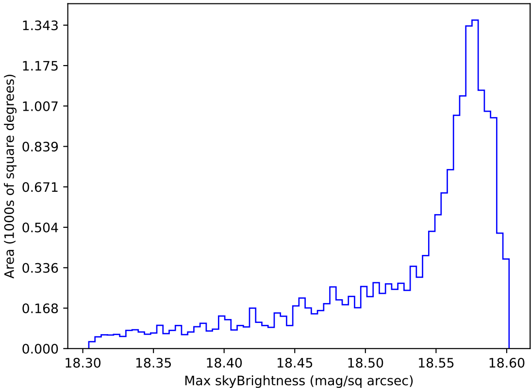
weather_cloudso4v3.4_10yrs WFD y band: Max skyBrightness
