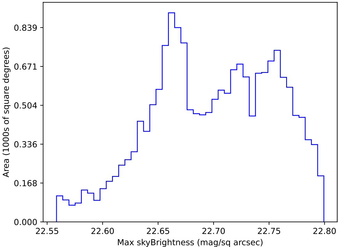
weather_cloudso4v3.4_10yrs WFD u band: Max skyBrightness
