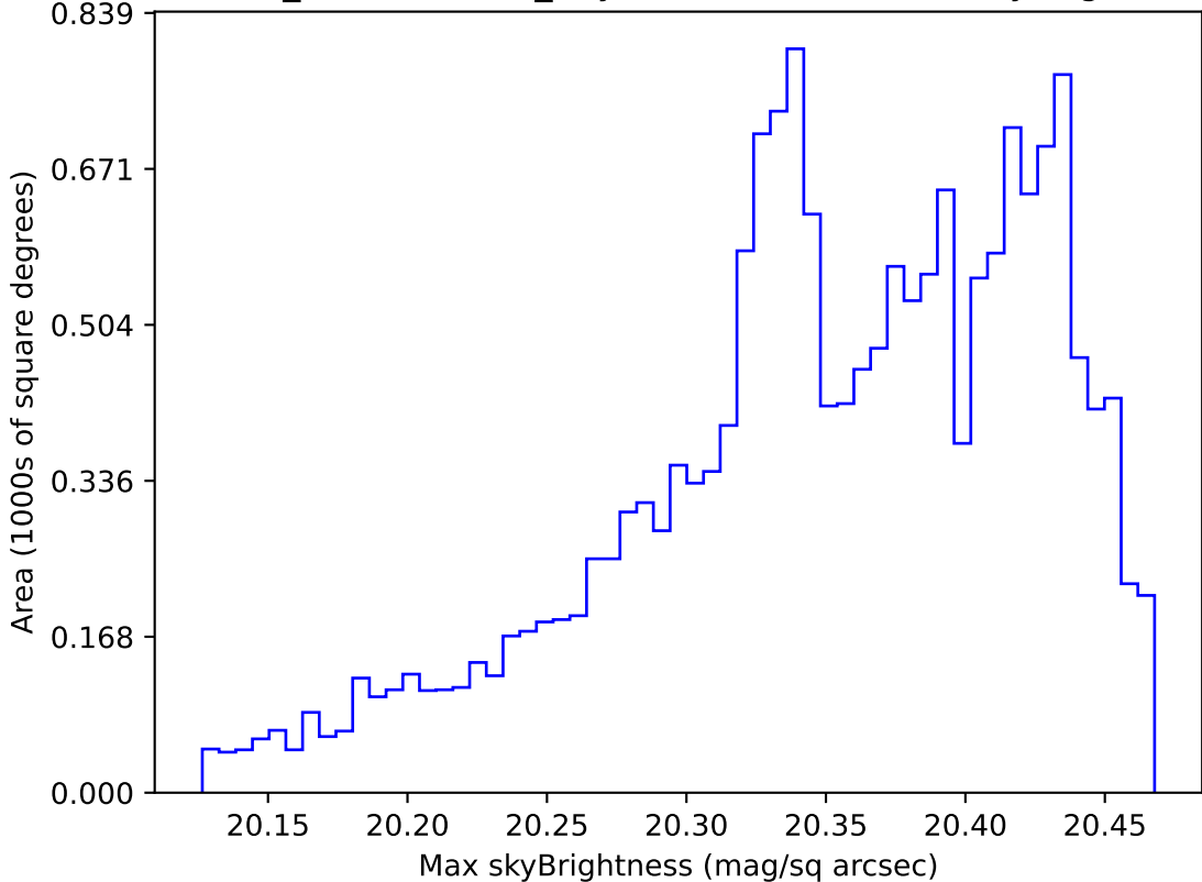
weather_cloudso4v3.4_10yrs WFD i band: Max skyBrightness
