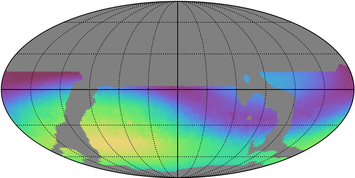
weather_cloudso4v3.4_10yrs WFD g band: Max skyBrightness
