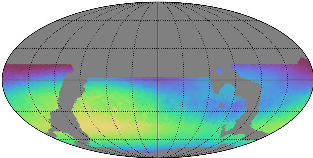
weather_cloudso4v3.4_10yrs WFD all bands: Max skyBrightness
