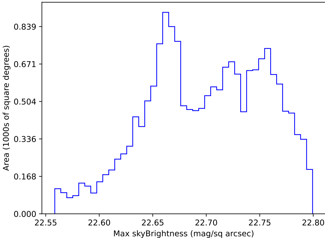
weather_cloudso4v3.4_10yrs WFD all bands: Max skyBrightness
