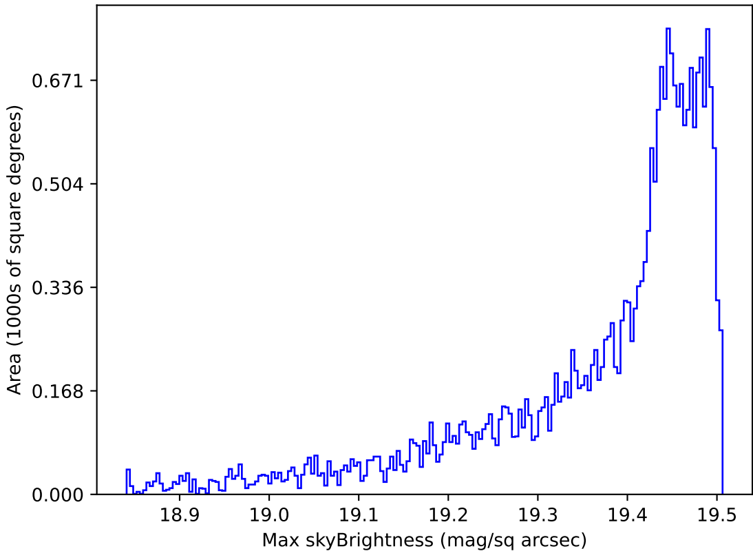
weather_cloudso4v3.4_10yrs All sky z band: Max skyBrightness
