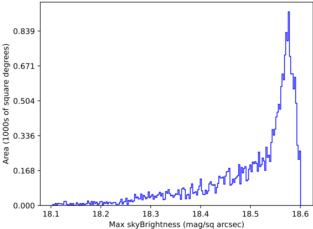
weather_cloudso4v3.4_10yrs All sky y band: Max skyBrightness
