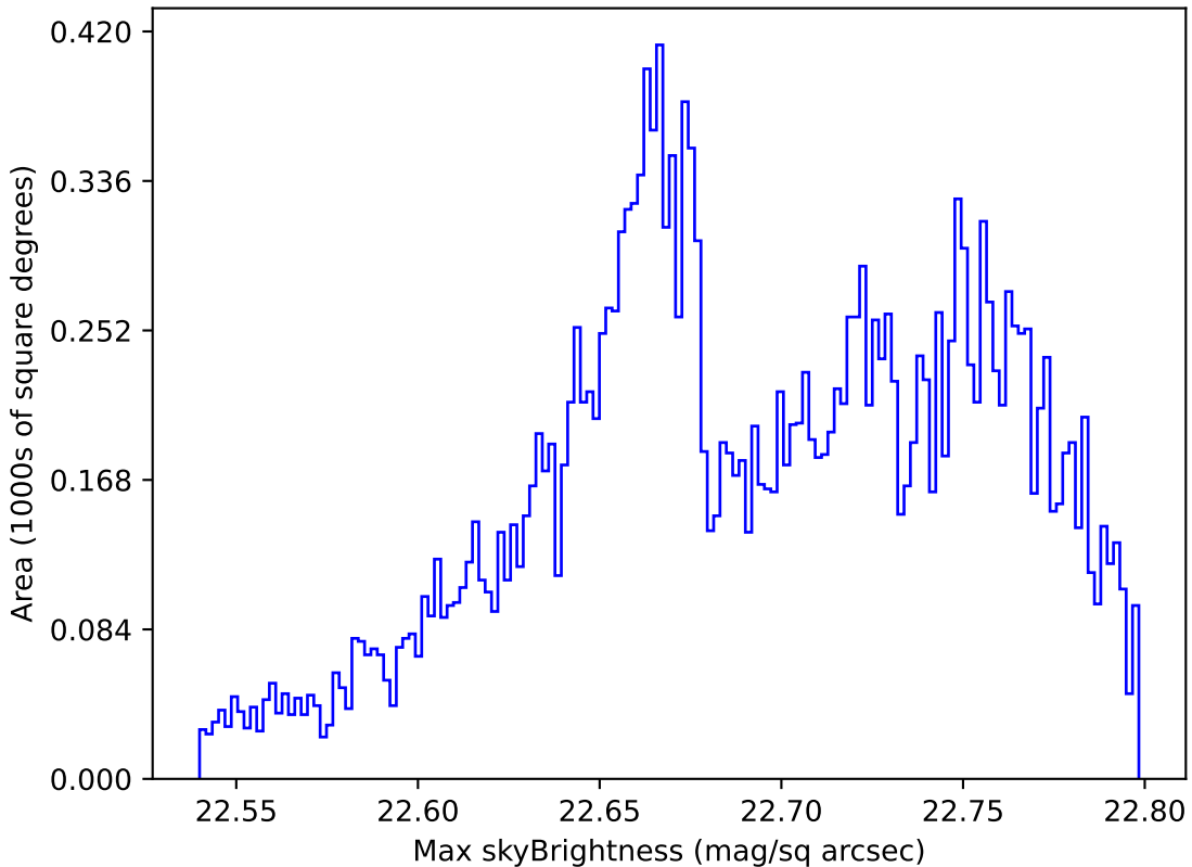
weather_cloudso4v3.4_10yrs All sky u band: Max skyBrightness
