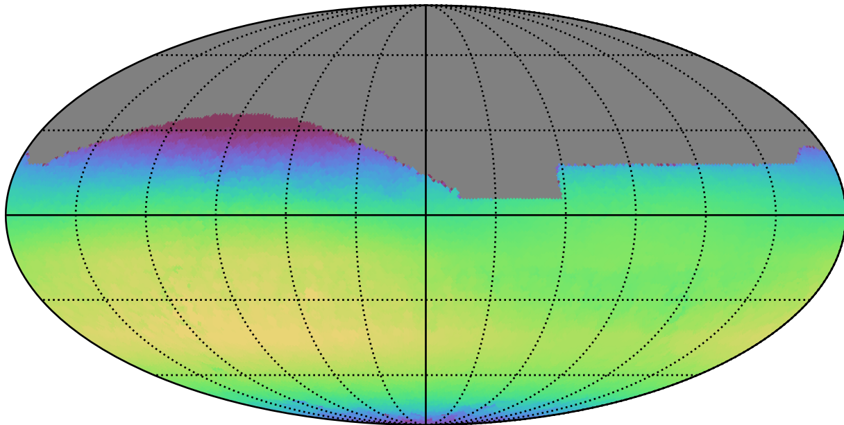
weather_cloudso4v3.4_10yrs All sky i band: Max skyBrightness
