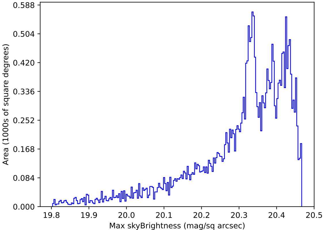
weather_cloudso4v3.4_10yrs All sky i band: Max skyBrightness
