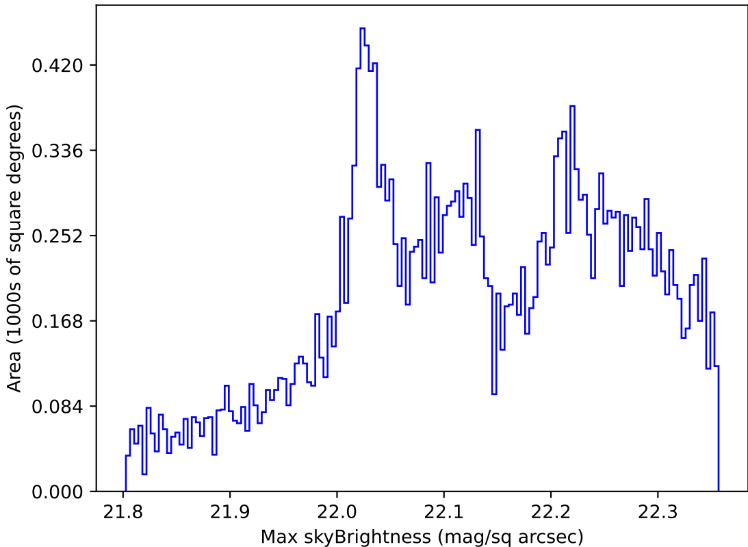
weather_cloudso4v3.4_10yrs All sky g band: Max skyBrightness
