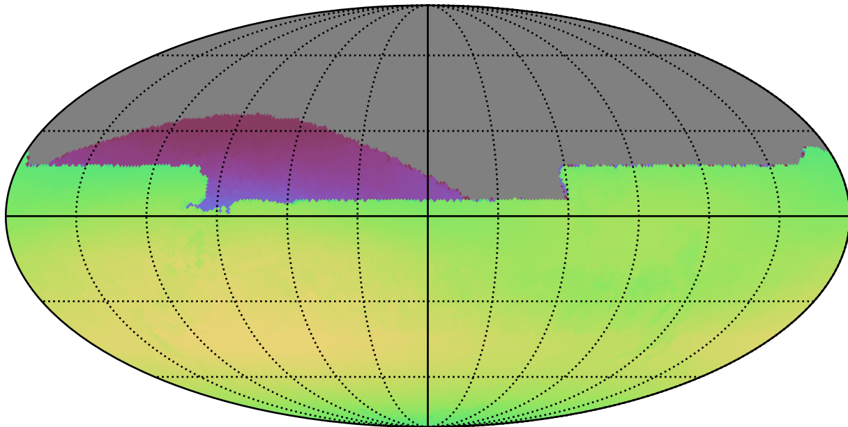
weather_cloudso4v3.4_10yrs All sky all bands: Max skyBrightness
