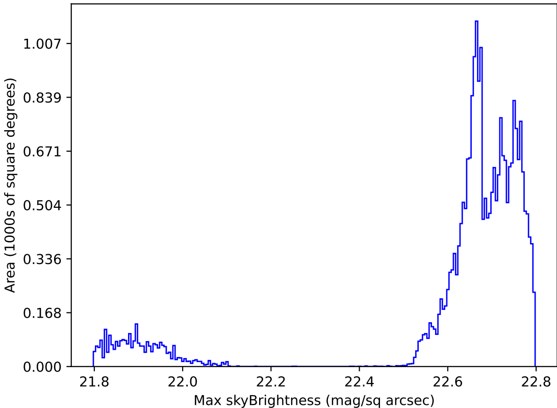
weather_cloudso4v3.4_10yrs All sky all bands: Max skyBrightness
