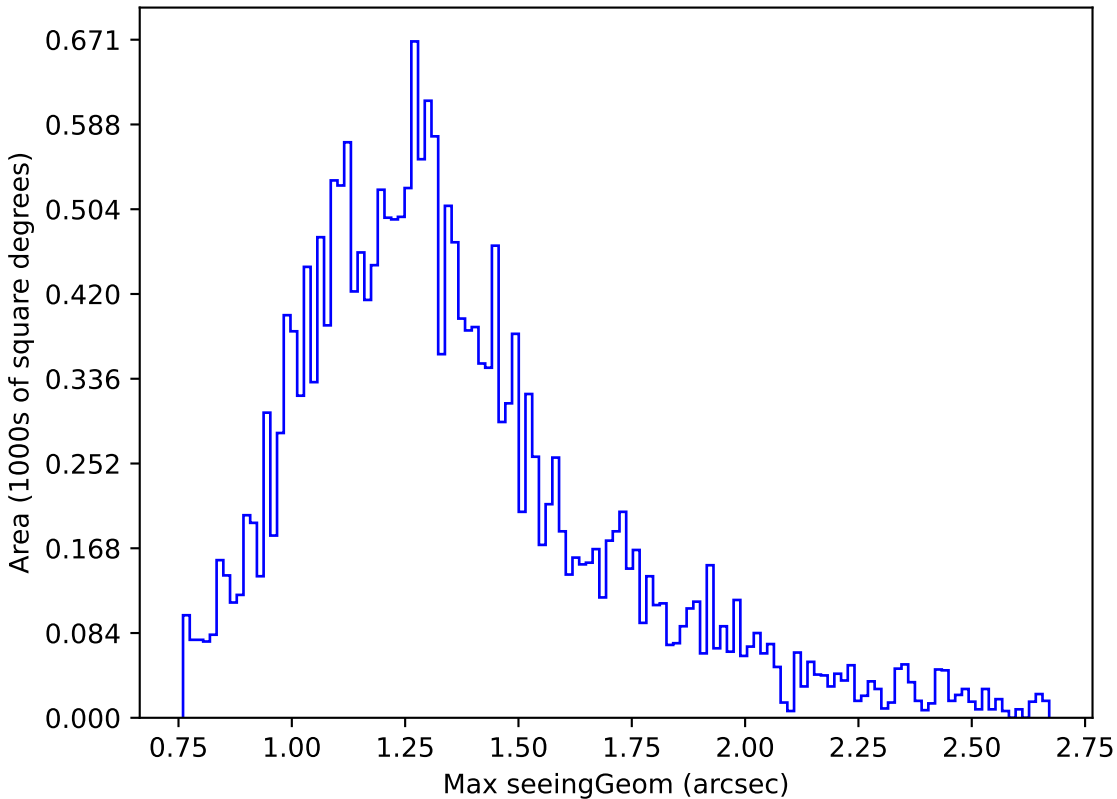
weather_cloudso4v3.4_10yrs Yr 1 u band: Max seeingGeom
