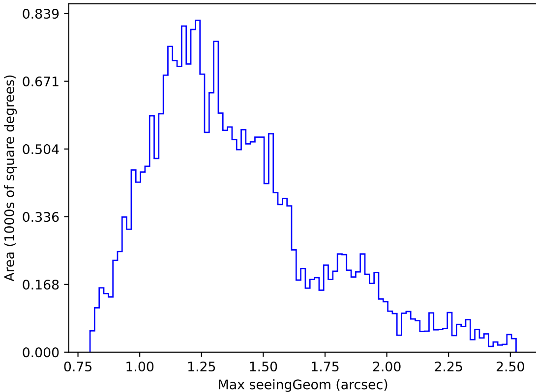
weather_cloudso4v3.4_10yrs Yr 1 i band: Max seeingGeom
