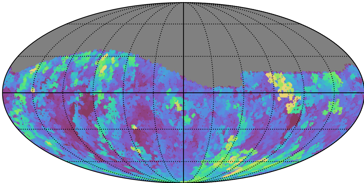
weather_cloudso4v3.4_10yrs Yr 1 g band: Max seeingGeom
