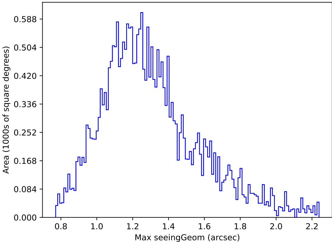
weather_cloudso4v3.4_10yrs Yr 1 g band: Max seeingGeom
