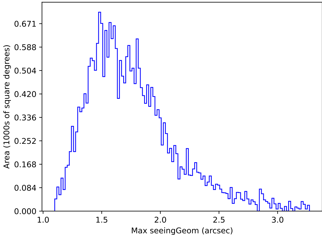
weather_cloudso4v3.4_10yrs Yr 1 all bands: Max seeingGeom
