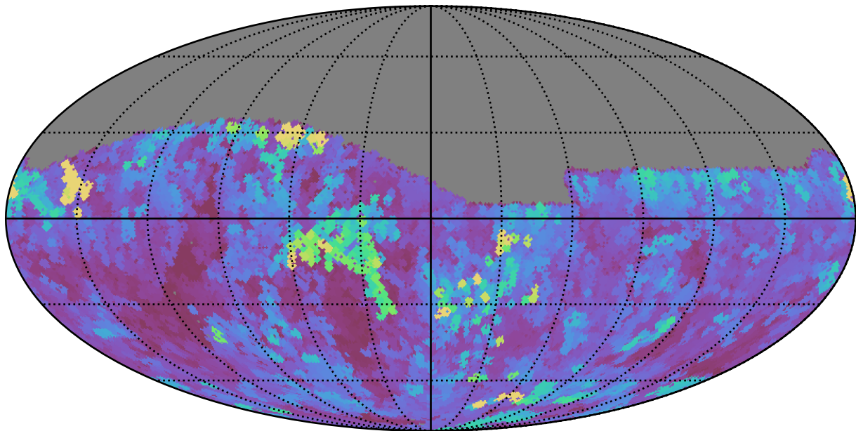
weather_cloudso4v3.4_10yrs Yr 1 z band: Max seeingEff
