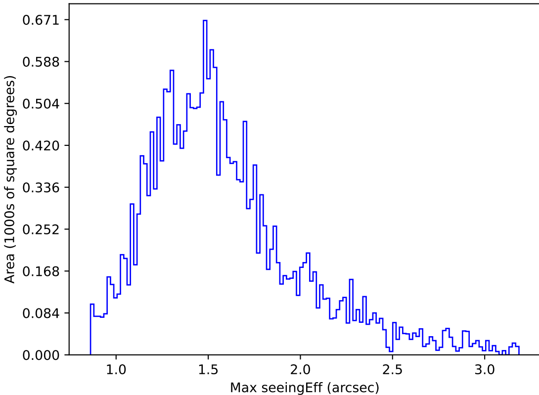
weather_cloudso4v3.4_10yrs Yr 1 u band: Max seeingEff
