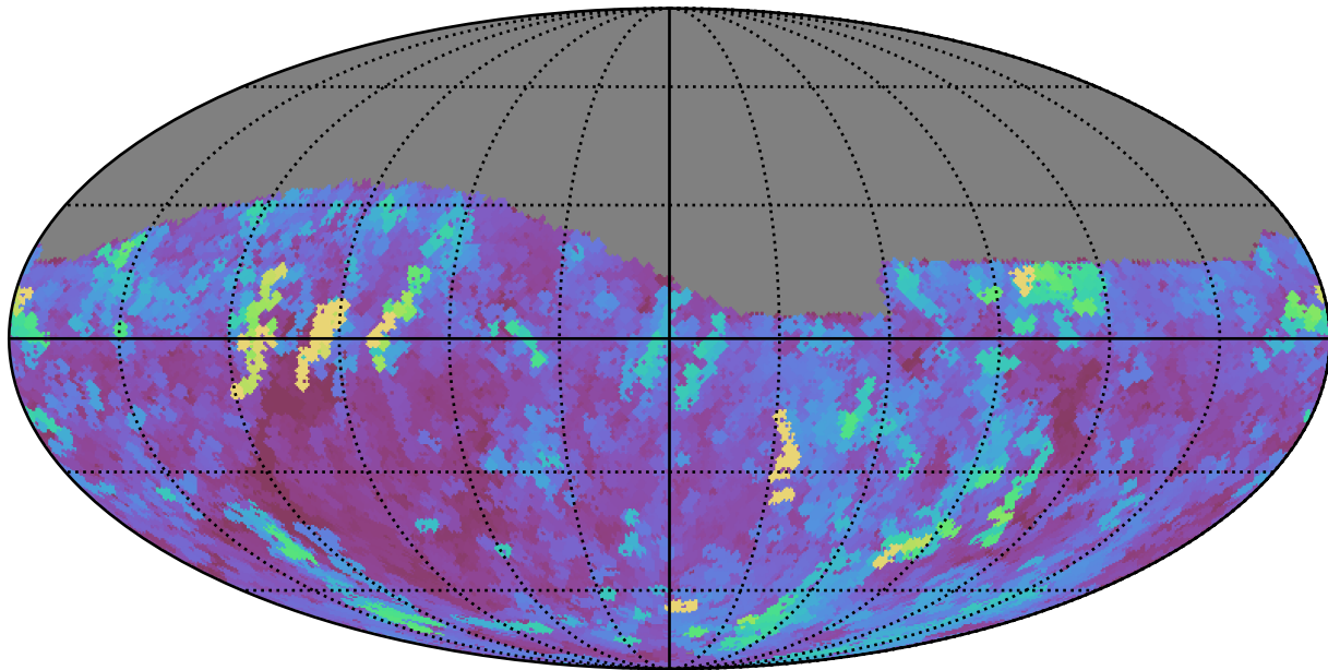
weather_cloudso4v3.4_10yrs Yr 1 r band: Max seeingEff
