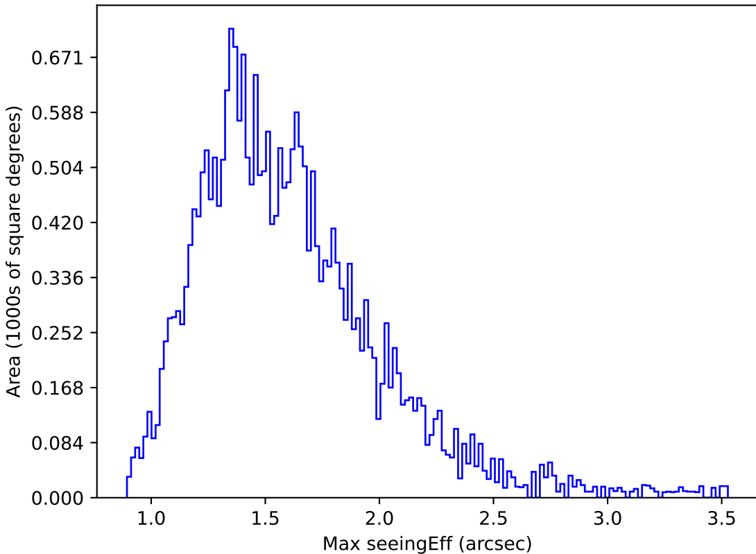
weather_cloudso4v3.4_10yrs Yr 1 r band: Max seeingEff
