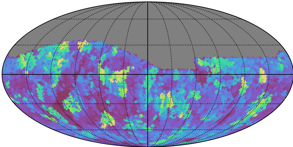
weather_cloudso4v3.4_10yrs Yr 1 i band: Max seeingEff
