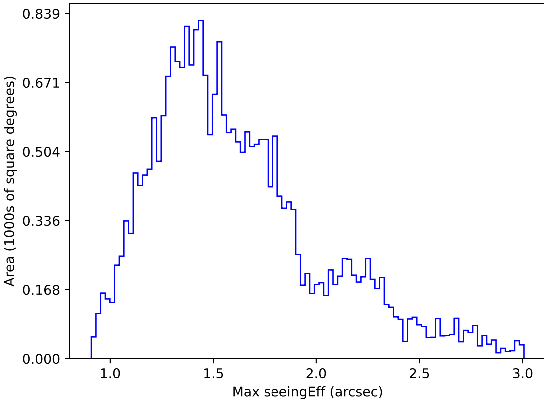
weather_cloudso4v3.4_10yrs Yr 1 i band: Max seeingEff
