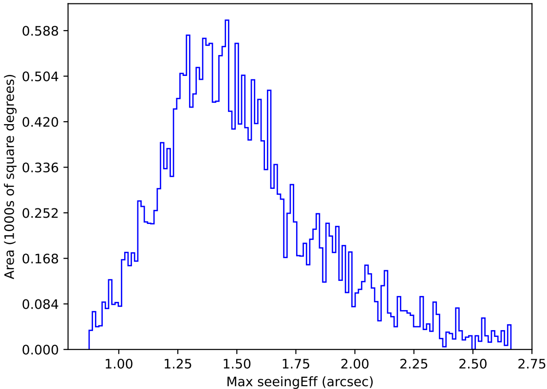
weather_cloudso4v3.4_10yrs Yr 1 g band: Max seeingEff
