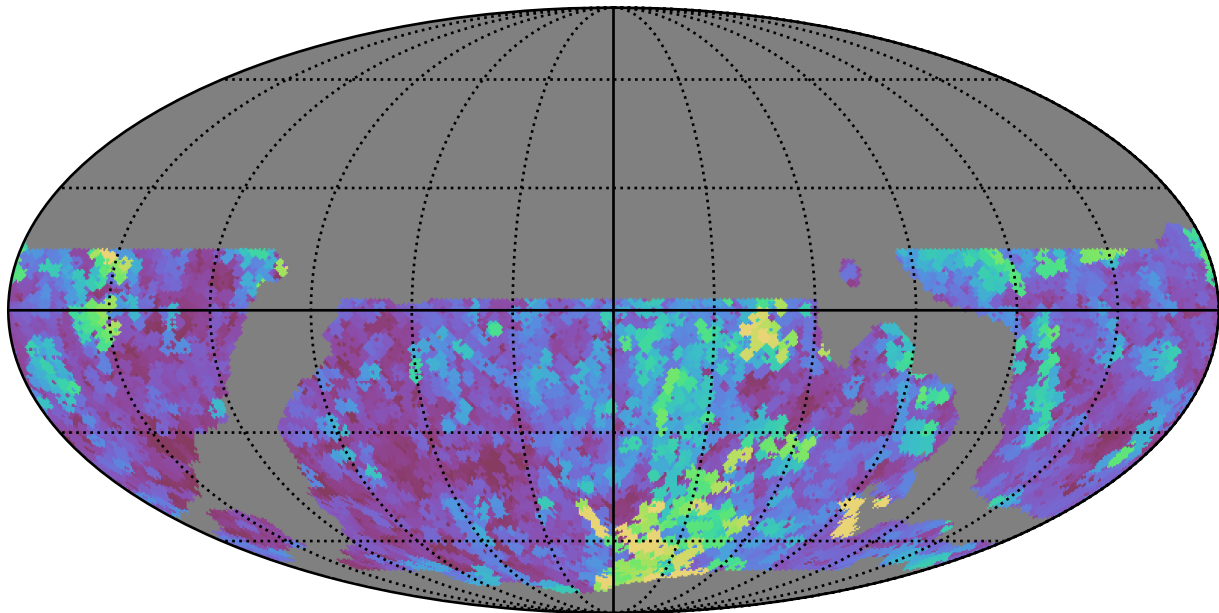
weather_cloudso4v3.4_10yrs WFD z band: Max seeingEff
