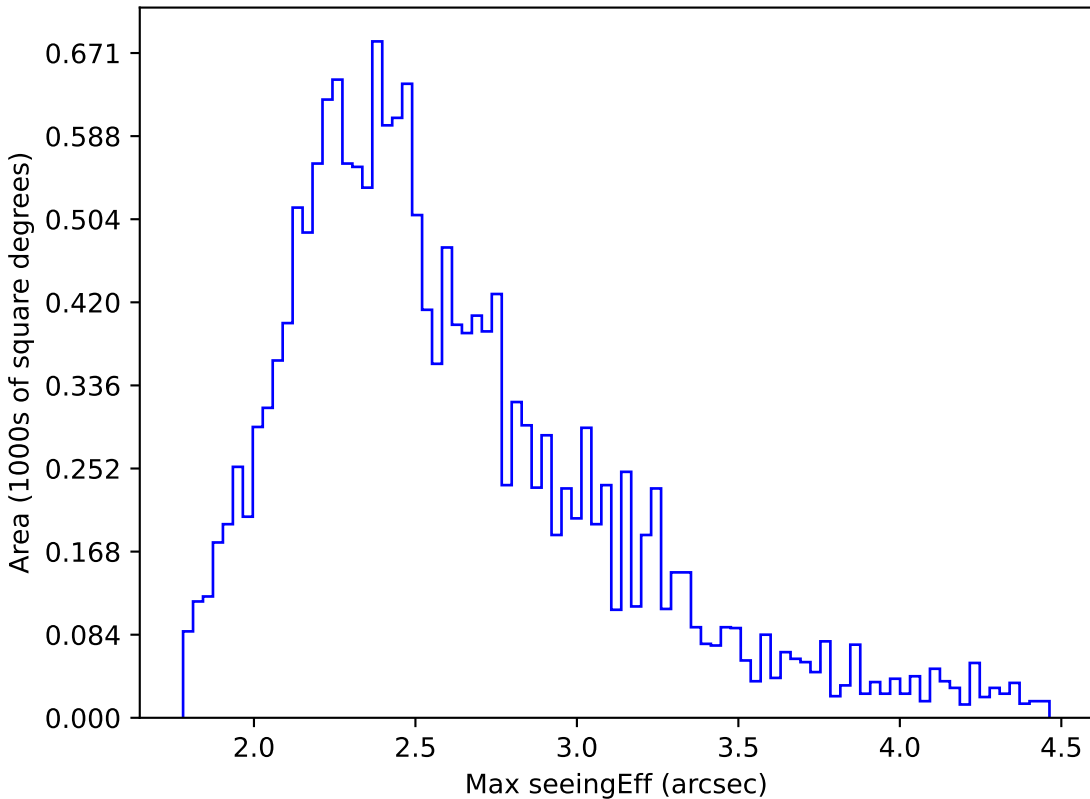
weather_cloudso4v3.4_10yrs WFD z band: Max seeingEff
