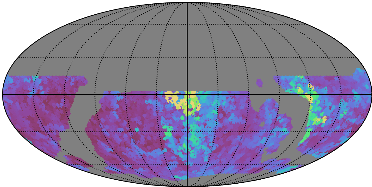
weather_cloudso4v3.4_10yrs WFD y band: Max seeingEff
