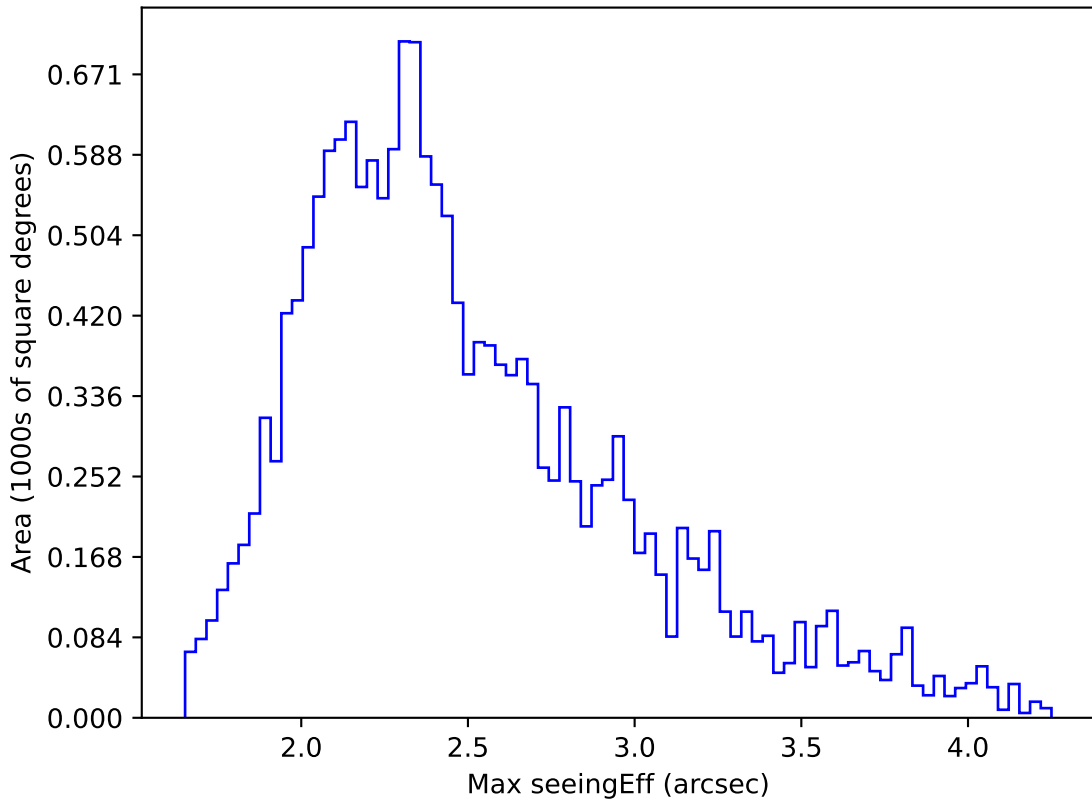
weather_cloudso4v3.4_10yrs WFD u band: Max seeingEff
