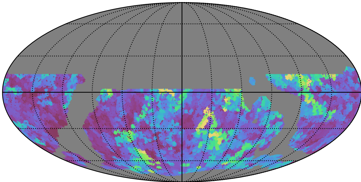
weather_cloudso4v3.4_10yrs WFD r band: Max seeingEff
