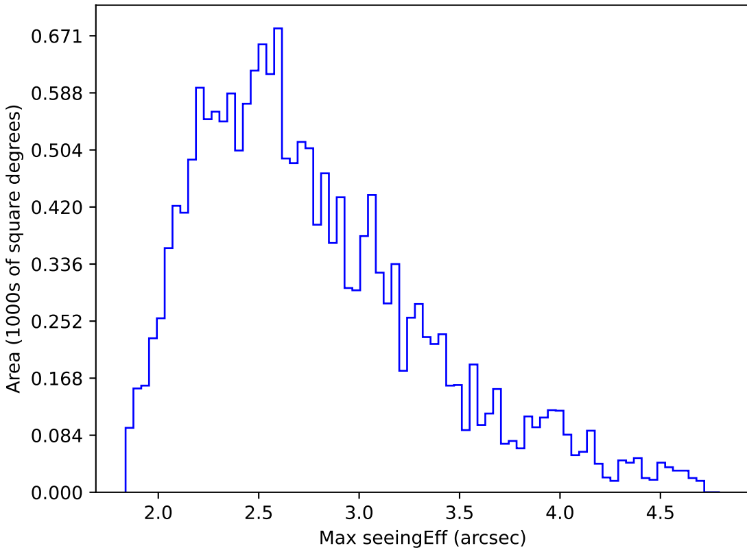
weather_cloudso4v3.4_10yrs WFD r band: Max seeingEff
