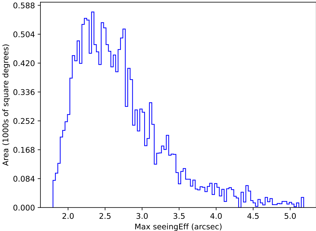
weather_cloudso4v3.4_10yrs WFD i band: Max seeingEff
