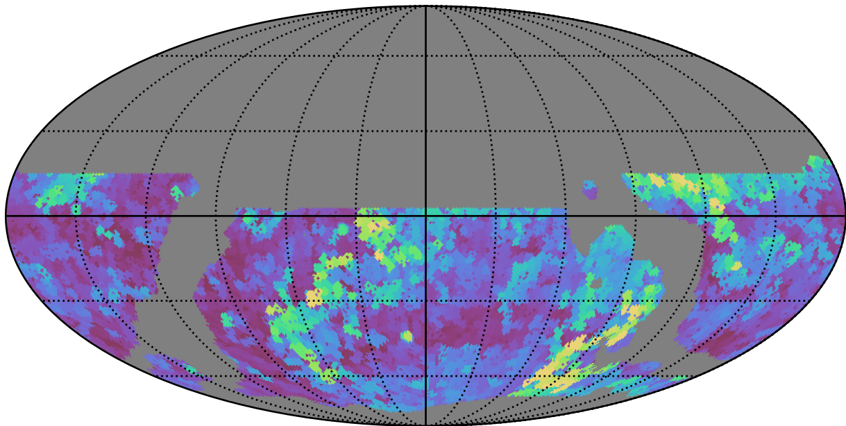
weather_cloudso4v3.4_10yrs WFD g band: Max seeingEff
