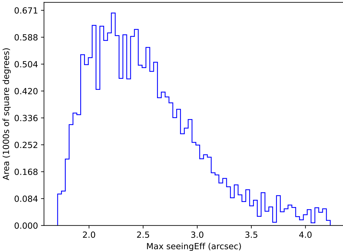
weather_cloudso4v3.4_10yrs WFD g band: Max seeingEff
