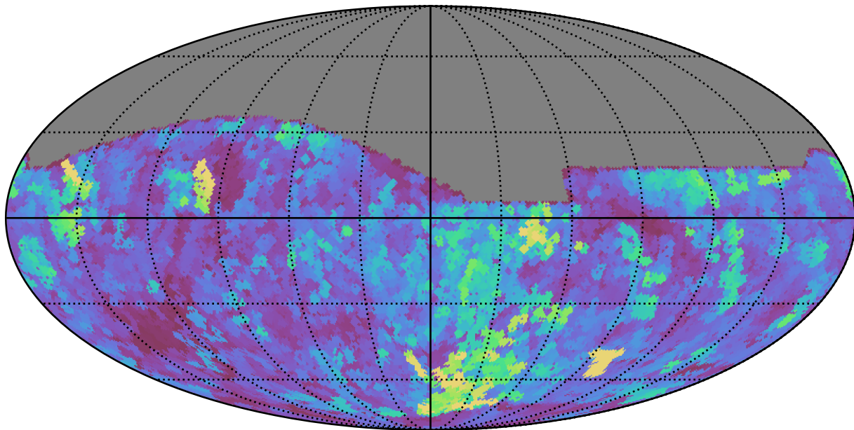
weather_cloudso4v3.4_10yrs All sky z band: Max seeingEff
