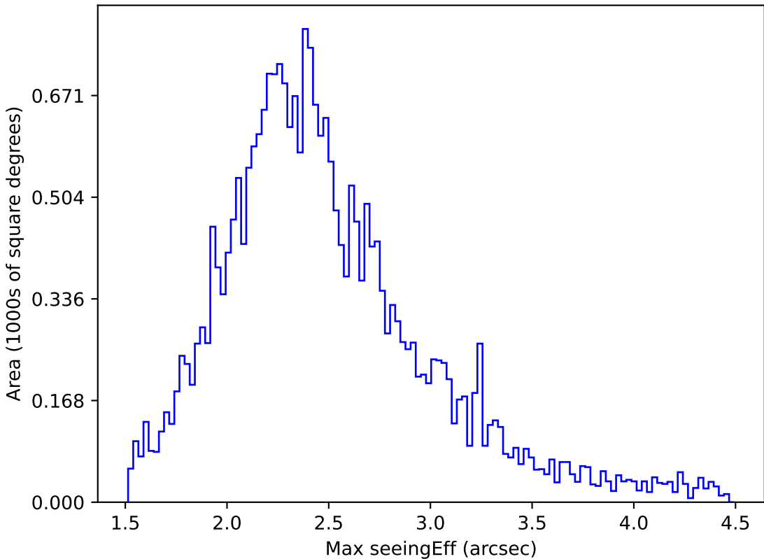
weather_cloudso4v3.4_10yrs All sky z band: Max seeingEff
