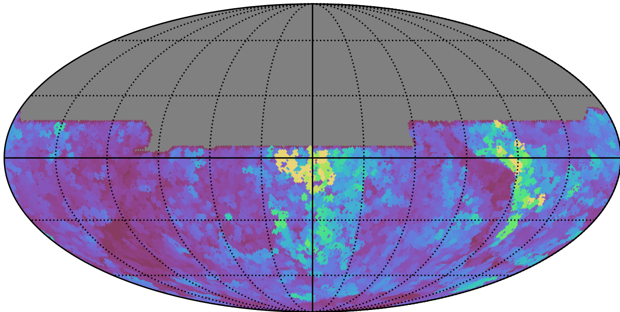
weather_cloudso4v3.4_10yrs All sky y band: Max seeingEff
