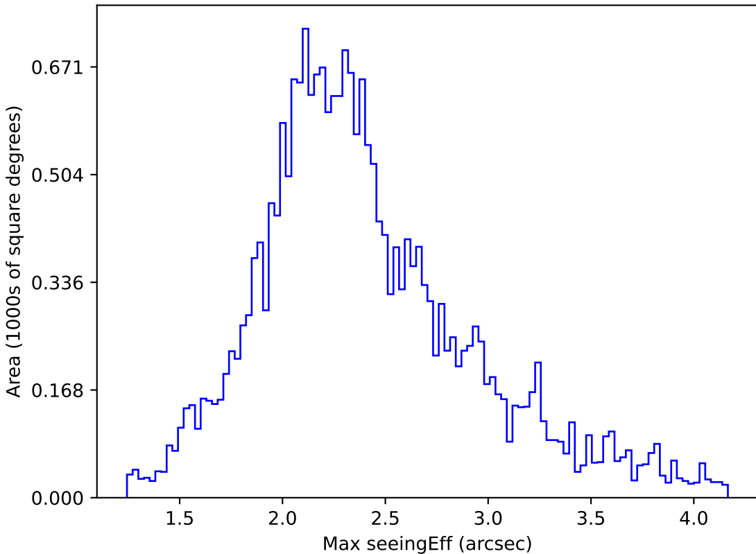
weather_cloudso4v3.4_10yrs All sky u band: Max seeingEff
