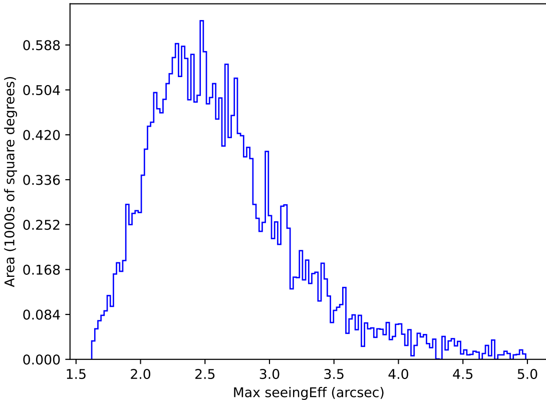
weather_cloudso4v3.4_10yrs All sky i band: Max seeingEff
