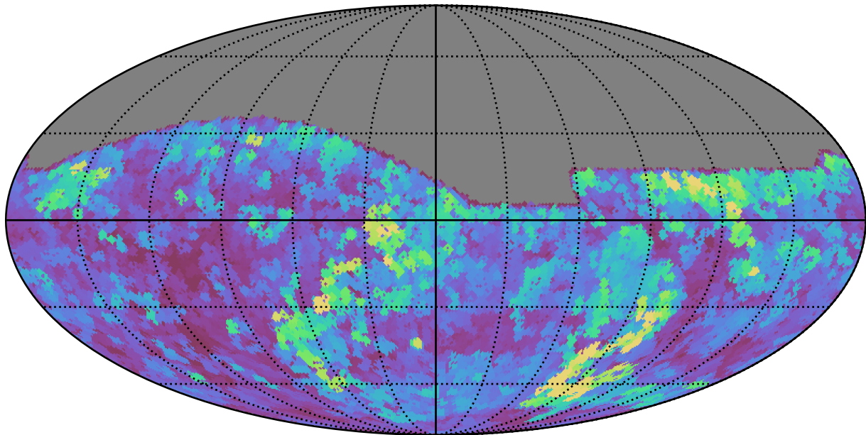
weather_cloudso4v3.4_10yrs All sky g band: Max seeingEff
