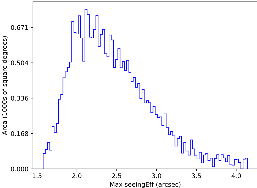
weather_cloudso4v3.4_10yrs All sky g band: Max seeingEff
