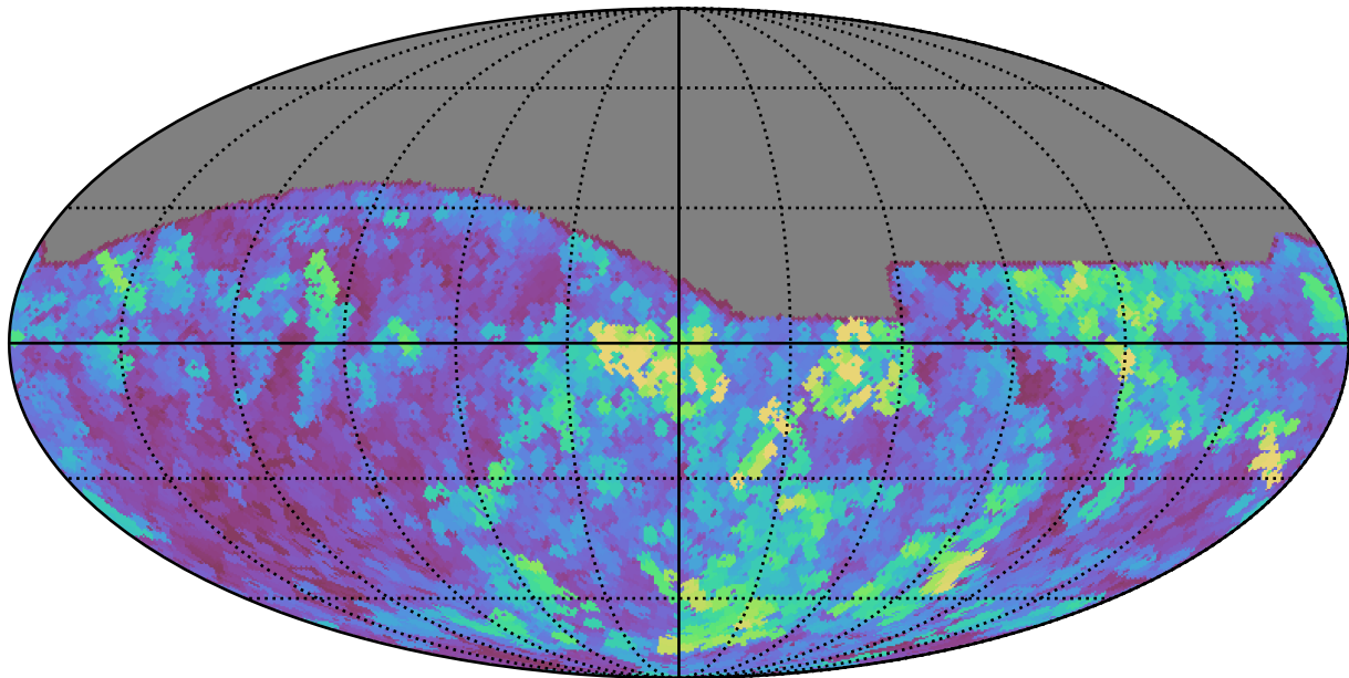
weather_cloudso4v3.4_10yrs All sky all bands: Max seeingEff
