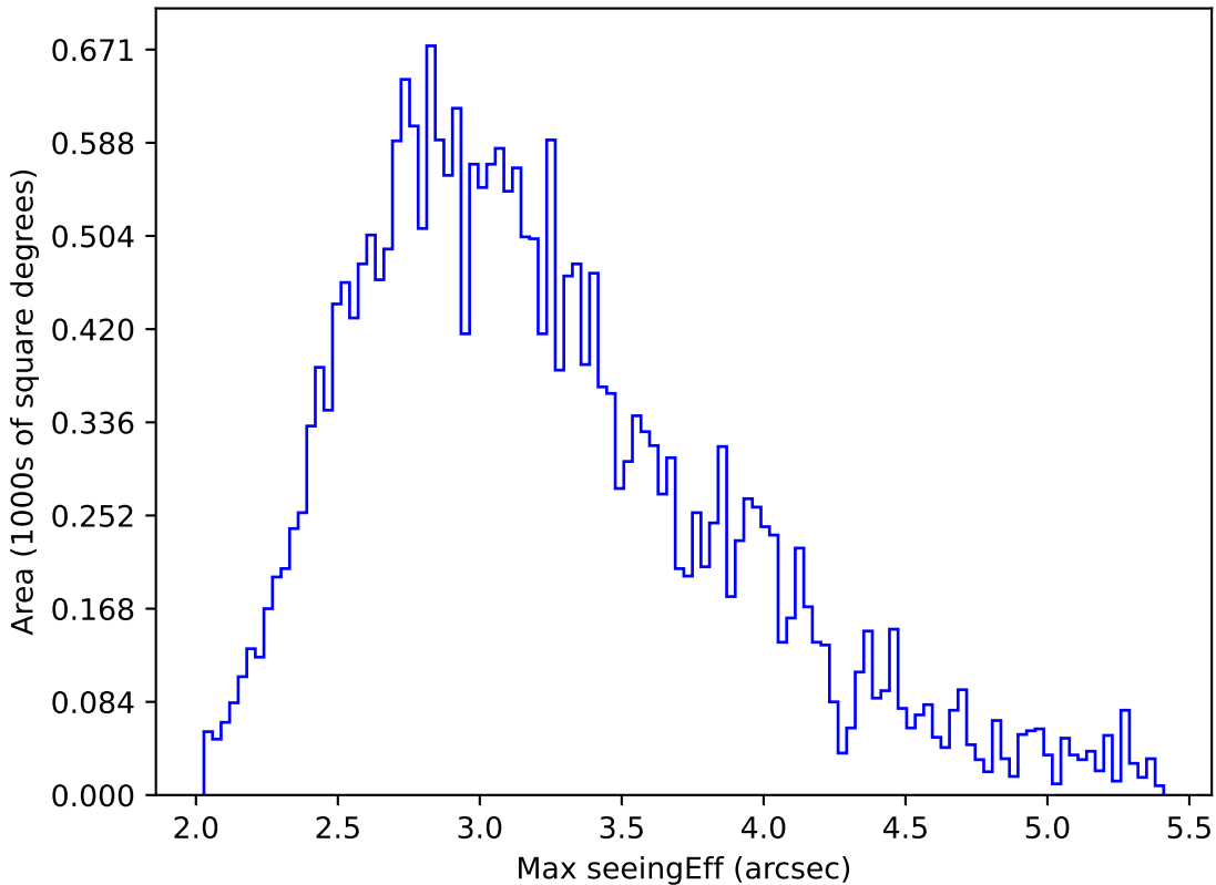
weather_cloudso4v3.4_10yrs All sky all bands: Max seeingEff
