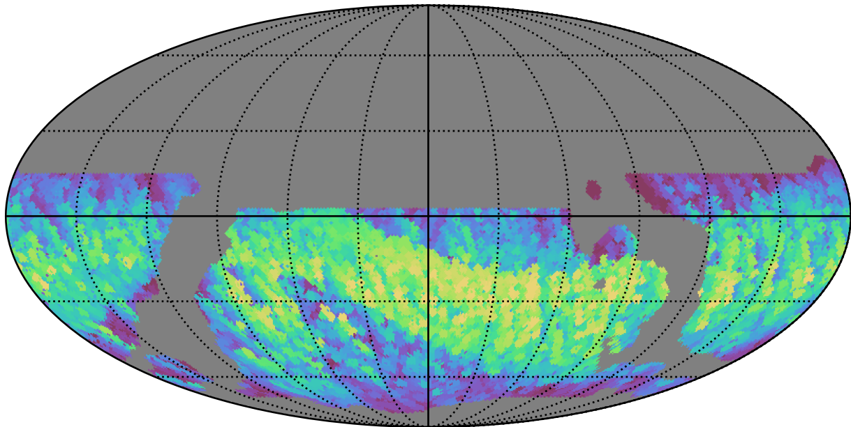
weather_cloudso4v3.4_10yrs WFD z band: Max normairmass
