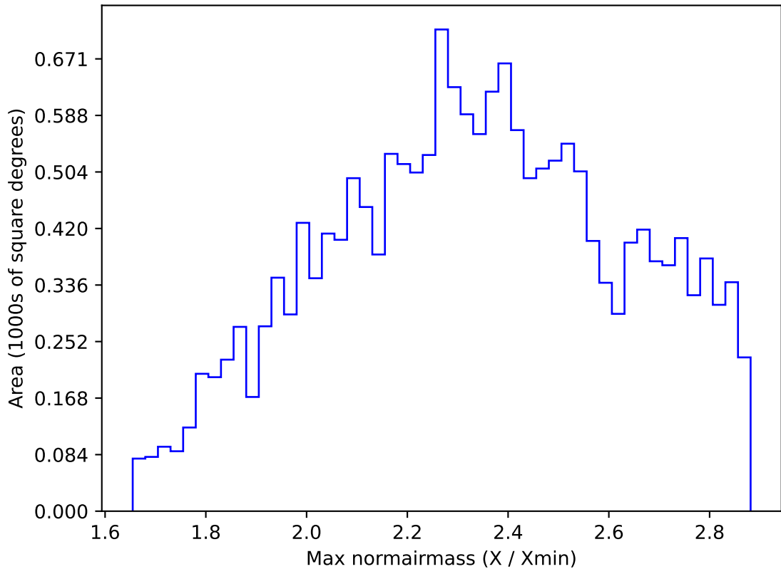
weather_cloudso4v3.4_10yrs WFD z band: Max normairmass
